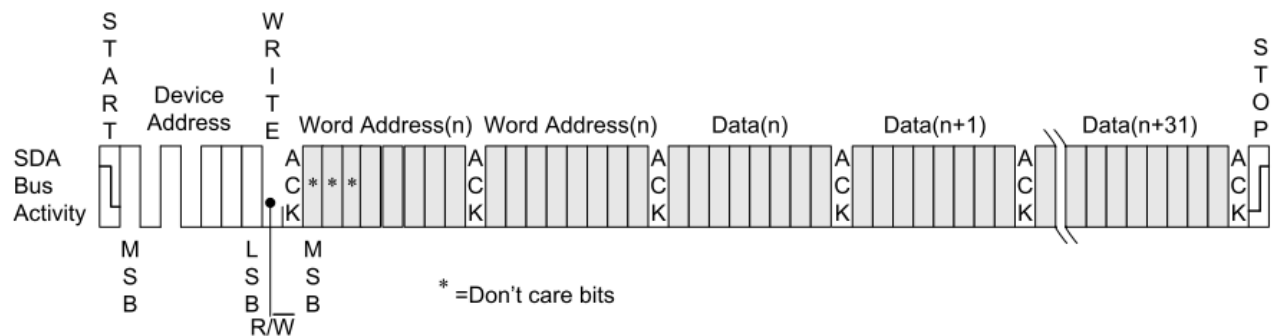
Figure 7. Page Write
