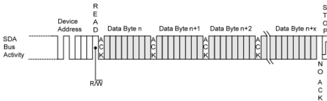
Figure 10. Sequential Read
