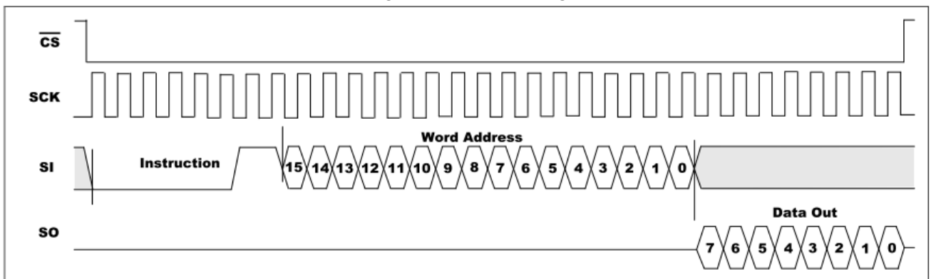
Figure 6. READ Timing
