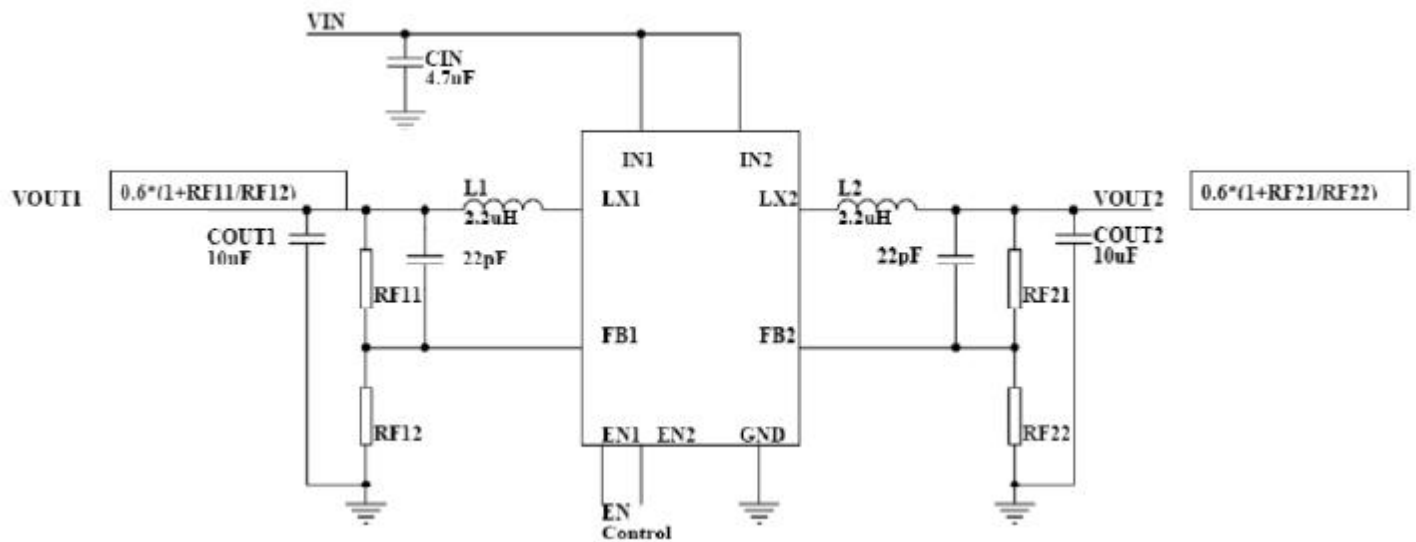
Figure 3. Type Application Circuit of EC3221
