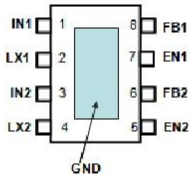
Figure 2 Pin Configuration of EC3221
