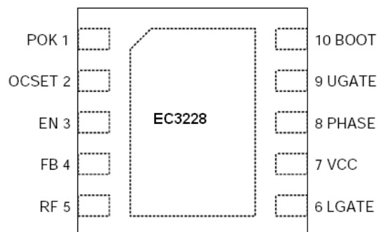
TDFN3x3-10 Top View
