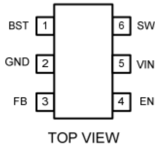
EC3292B Top View
