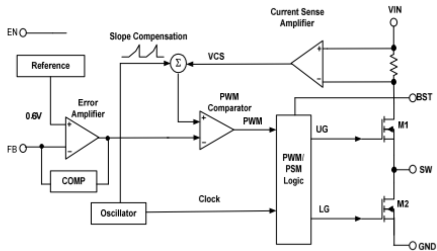
Figure 2. EC3292B Functional Block Diagram
