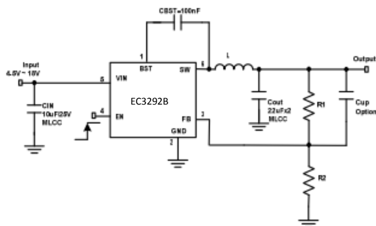
Figure 1. EC3292B Typical Operating Circuit
