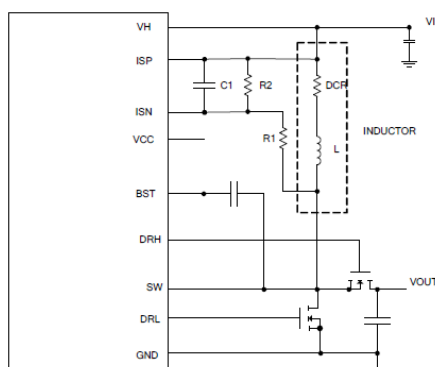
(4b) Using the Inductor DCR to Sense Current
