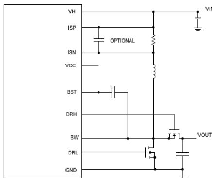
(4a) Using a Current Sense Resistor
