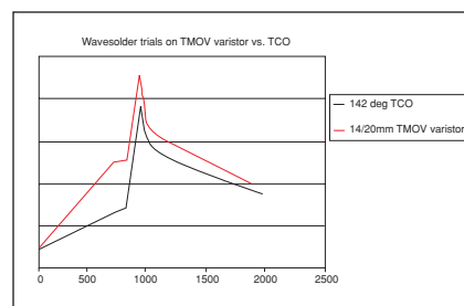
Figure 7. Wave solder profile of TMOV varistor vs. TCO (Tf=142°C)
