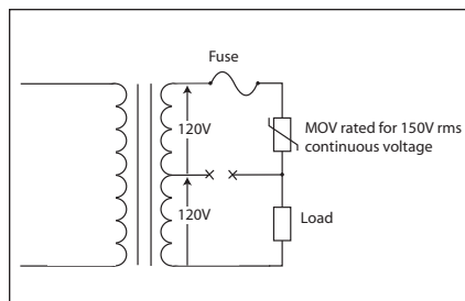
Figure 1. Possible Fault Condition for a limited current abnormal overvoltage event
