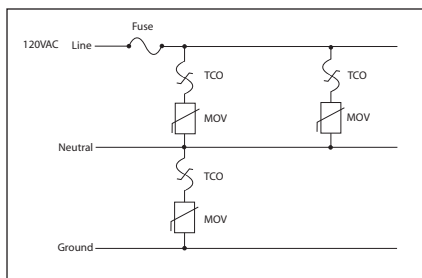
Figure 2. Typical offline protection scheme
