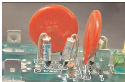
Figure 3. Typical Arrangement of TCOs with MOVs ** one of the MOVs has been removed for clarity
