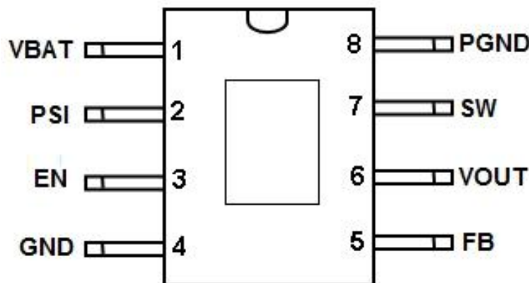
Figure 1 Pin Configuration of EC9288(Top View)
