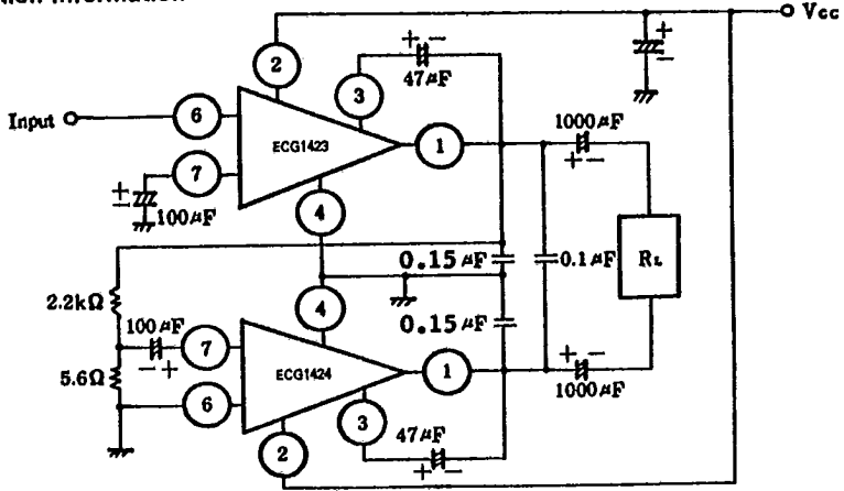
BTL (Balanced Transformerless) Application Example
