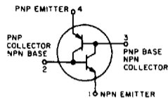
Transistor Equivalent Circuit
