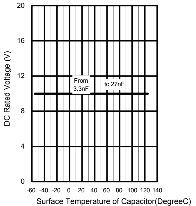
Voltage Derating by Temperature
