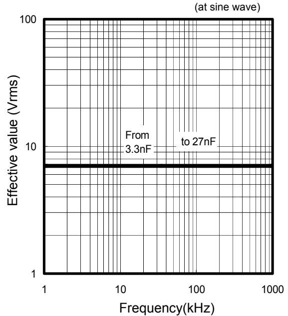
Permissible Voltage
