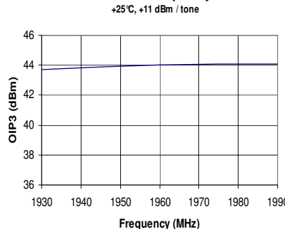
OIP3 vs. Frequency
