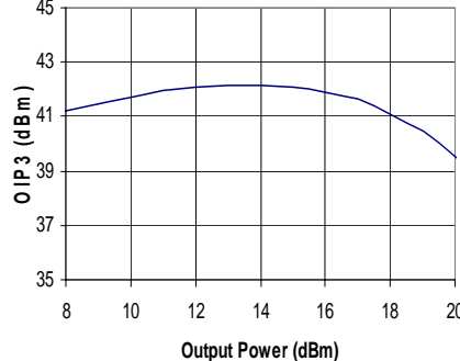
OIP3 vs. Output Power
