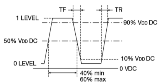
Figure 3) HCMOS Output Wave Form
