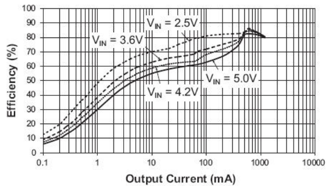
Efficiency vs. Output Current ( V_{OUT} = 1.2V ; T_A = 25^\circ C ; L = 2.2\mu H )
