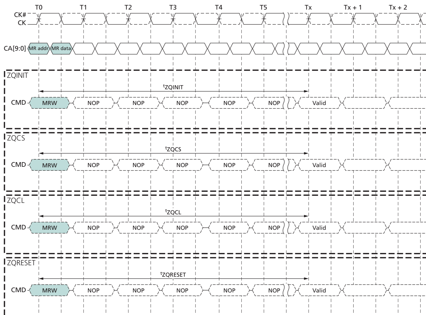
Figure 43: ZQ Timings
