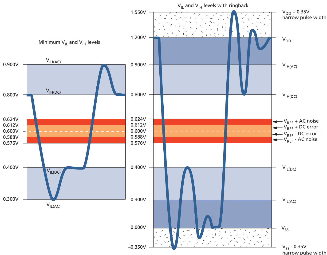
Figure 60: LPDDR2-200 to LPDDR2-400 Input Signal
