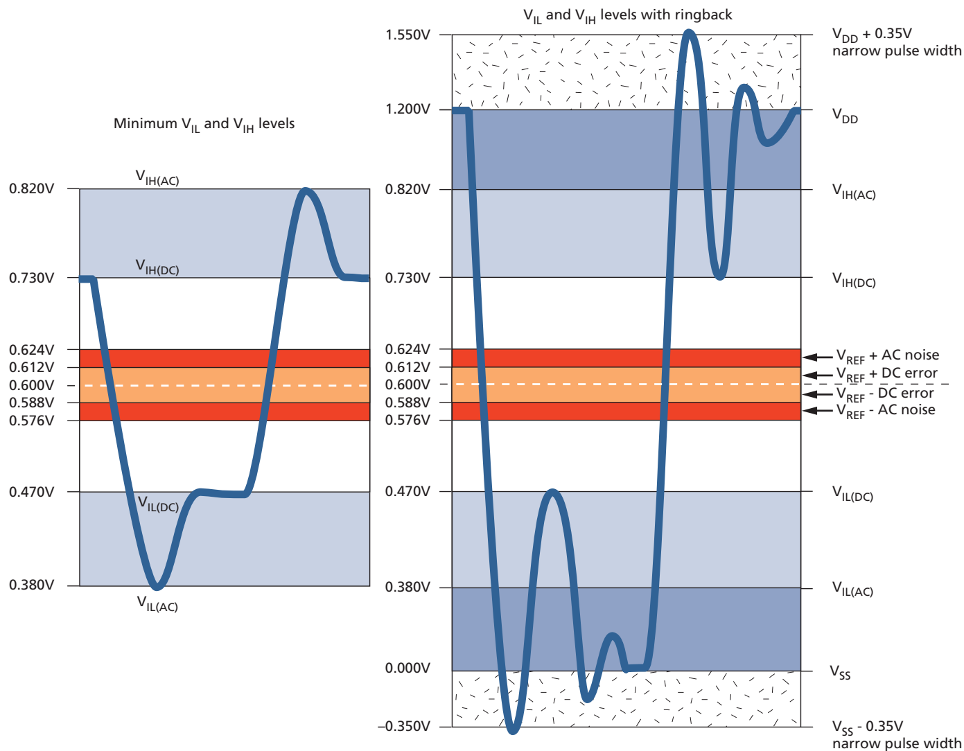
Figure 59: LPDDR2-466 to LPDDR2-1066 Input Signal
