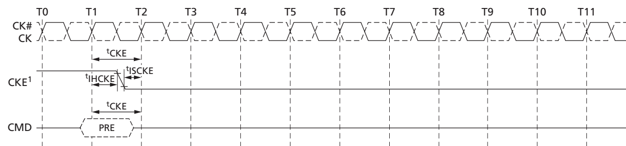
Figure 53: PRECHARGE Command to Power-Down Entry
