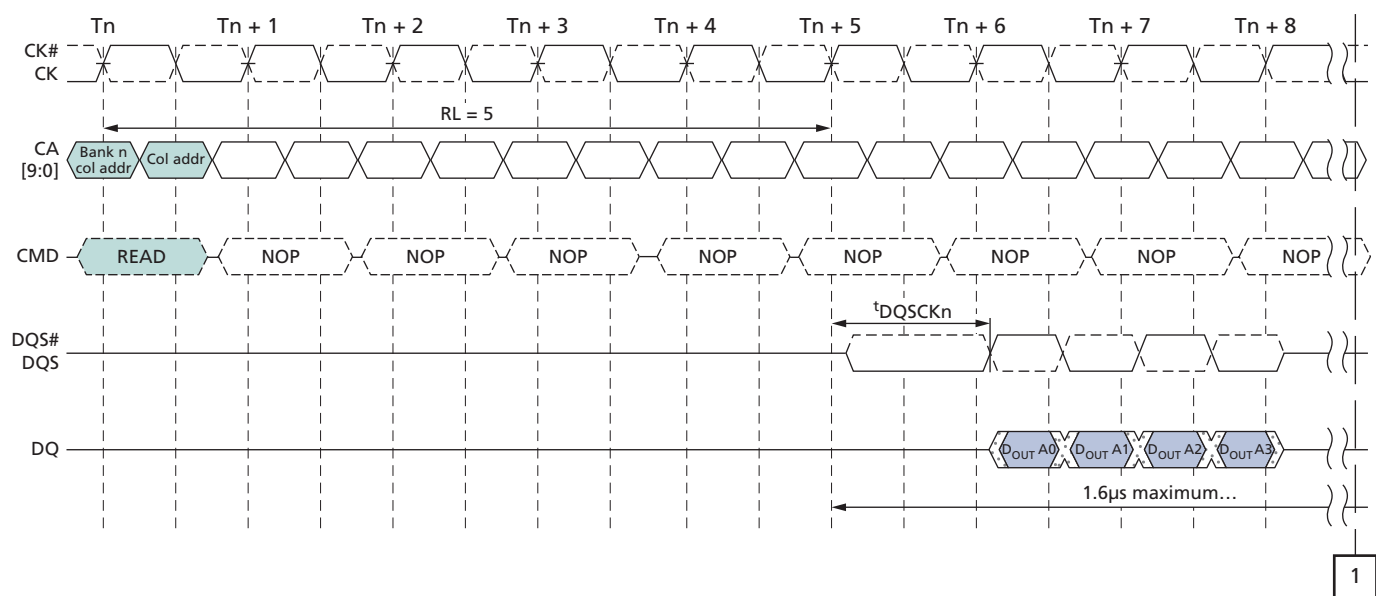
Figure 17: t_{DQCKDM} Timing
