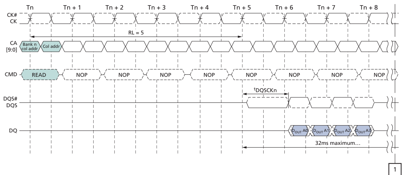
Figure 16: t_{DQSKDL} Timing
