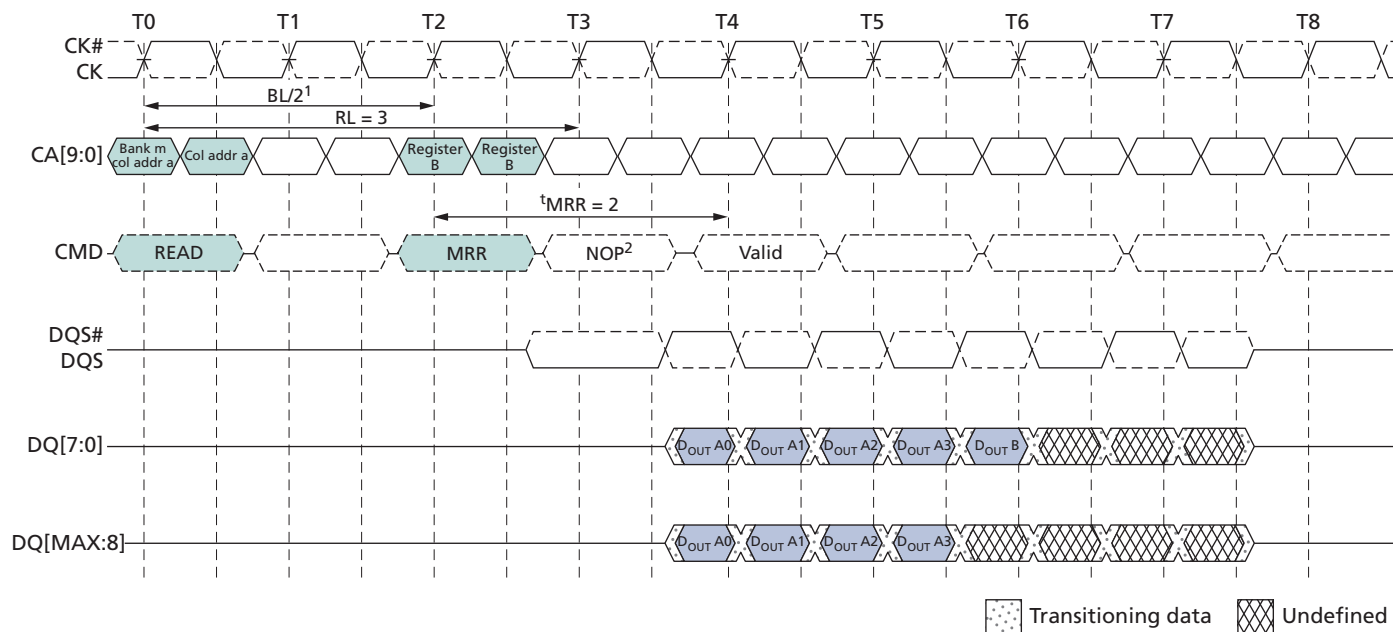
Figure 38: READ to MRR Timing – RL = 3, t_{MRR} = 2
