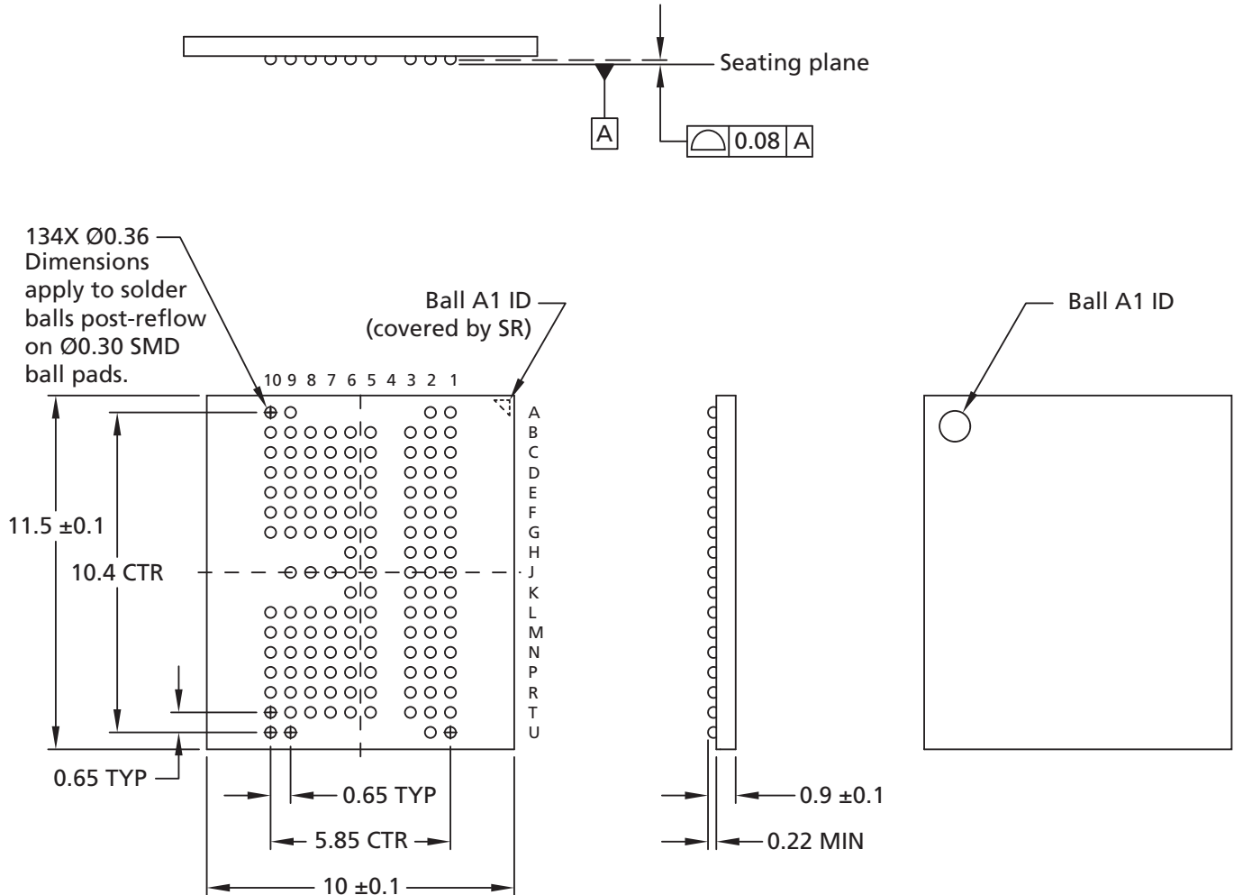
Figure 5: 134-Ball VFBGA – 10mm x 11.5mm (Package Code: BH)
