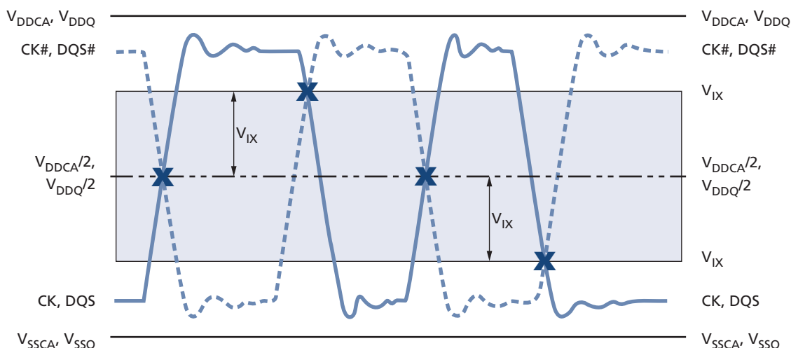
Figure 63: V_{IX} Definition
