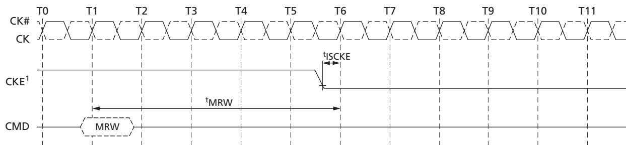
Figure 55: MRW Command to Power-Down Entry
