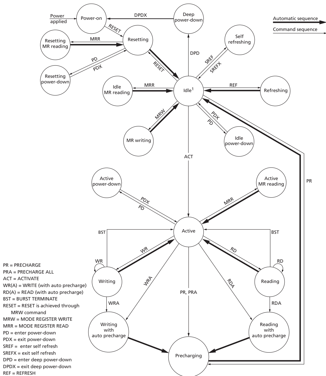
Figure 57: Simplified Bus Interface State Diagram
