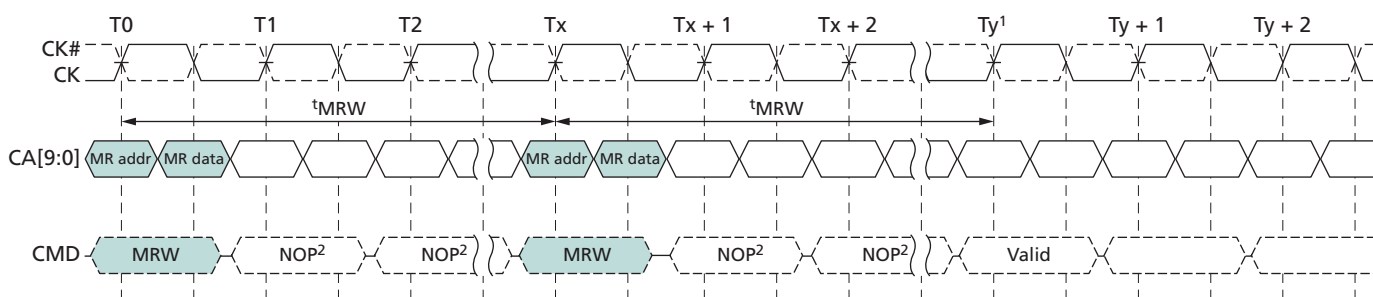
Figure 42: MODE REGISTER WRITE Timing – RL = 3, t_{MRW} = 5
