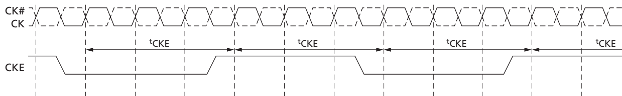
Figure 45: CKE Intensive Environment
