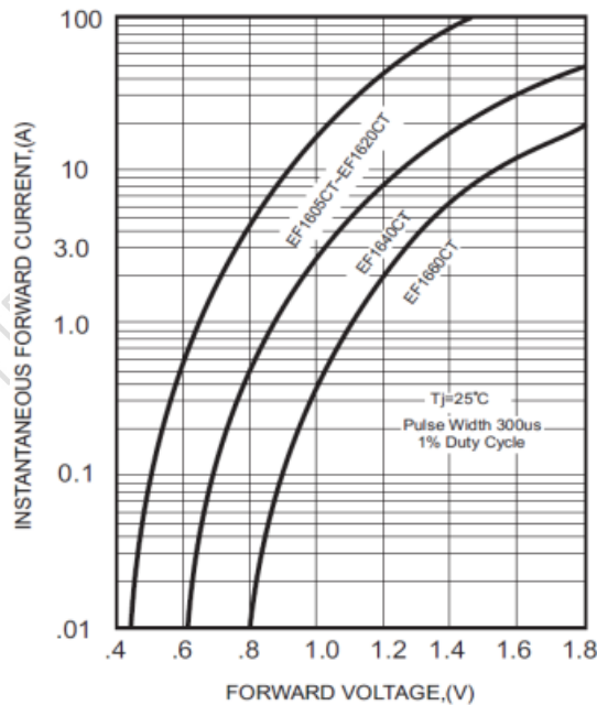
FIG.3-TYPICAL FORWARD CHARACTERISTICS
