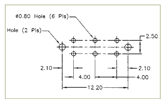
P.C. MOUNTING
