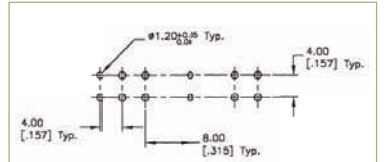
P.C. MOUNTING
