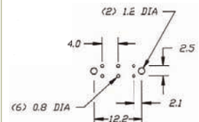
P.C. MOUNTING
