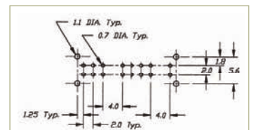
P.C. MOUNTING
