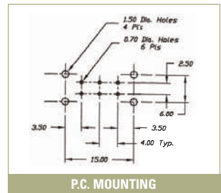
P.C. MOUNTING
