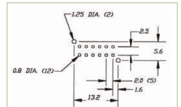
P.C. MOUNTING
