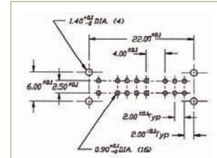
P.C. MOUNTING
