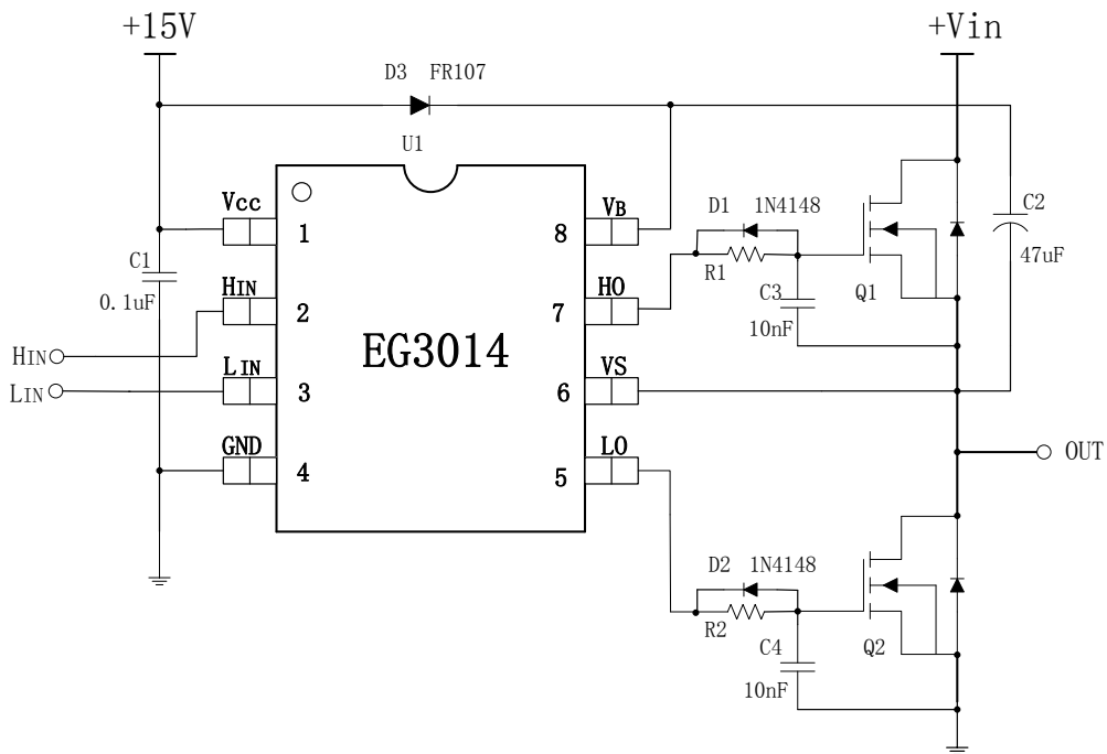
Fig 6-3. EG3014 typical application schematic III for external bootstrap diode
