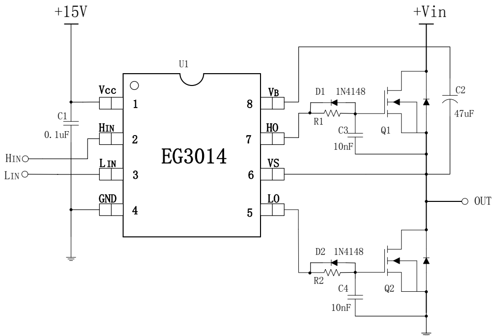
Fig 6-1. EG3014 typical application schematic I for middle power motor
