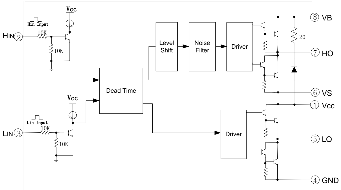
Fig 5-1. EG3014 block diagram
