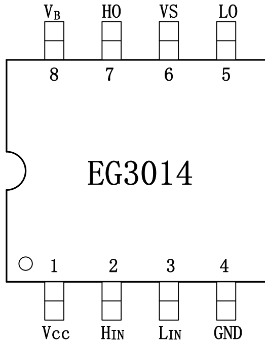
Figure 4-1. EG3014 pin map
