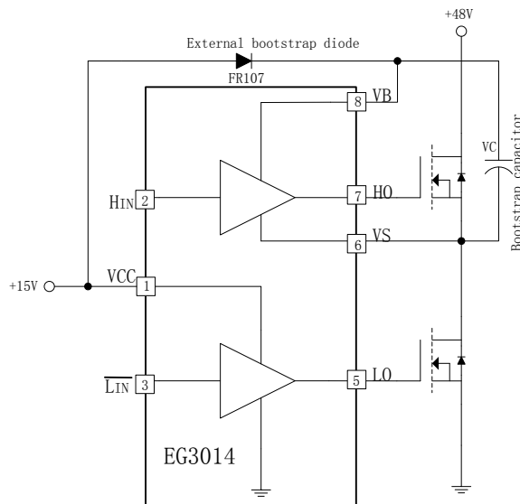
Figure 8-3. EG3014 Bootstrap circuit structure
