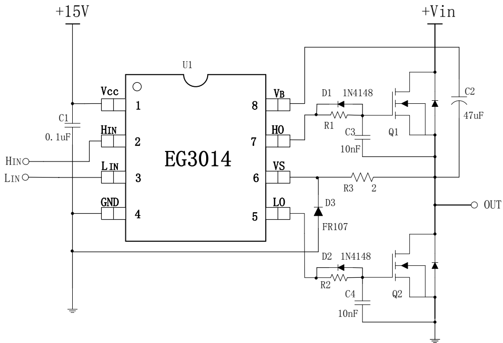
Fig 6-2. EG3014 typical application schematic II for high power motor
