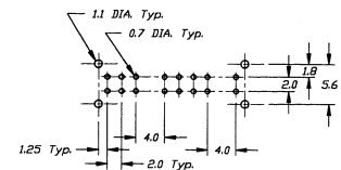
P.C. MOUNTING
