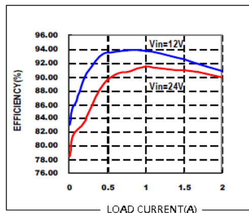
Efficiency vs Load Current (Vout = 5V)
