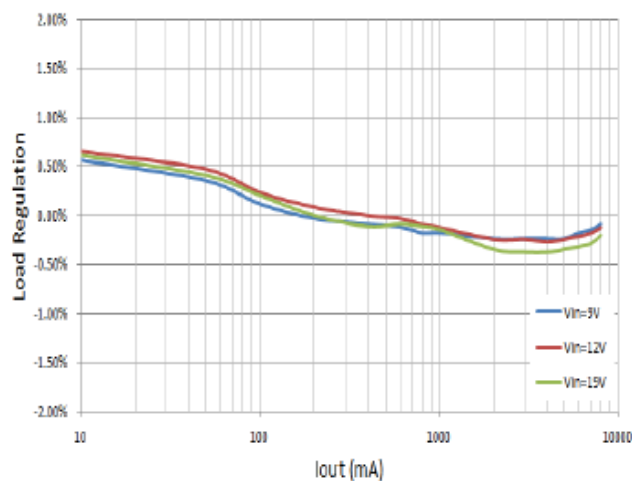
Figure 3. Load regulation vs Load Current (V out =3.3V, L=1.5uH)
