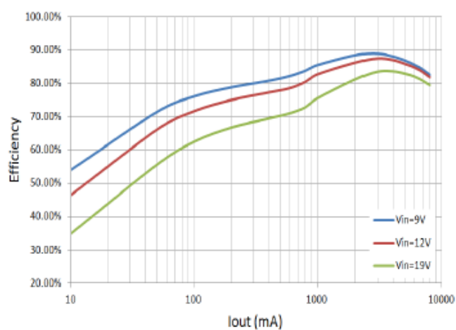
Figure 2. Efficiency vs Load Current (V out =1V, L=1uH)
