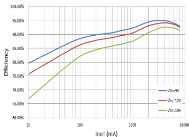
Figure 1. Efficiency vs Load Current (V out =3.3V, L=1.5uH)
