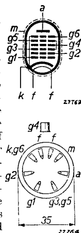
Fig. 2 Arrangement of electrodes and base connections.
