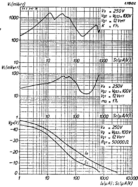
Fig. 7 Upper diagram. Alternating input voltage as a function of the conversion conductance controlled by the bias on grid 4, with 1 % cross-modulation. Centre diagram. Alternating input voltage as a function of the conversion conductance controlled by the bias on grid 4, with 1 % modulation hum. Lower diagram. Anode current and conversion conductance as a function of the bias on grid 4.
