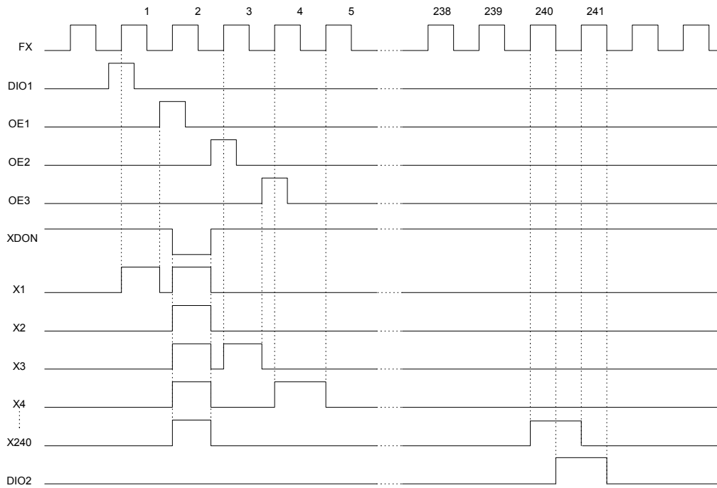
Fig. 5 XDON Functionality RL="H"
