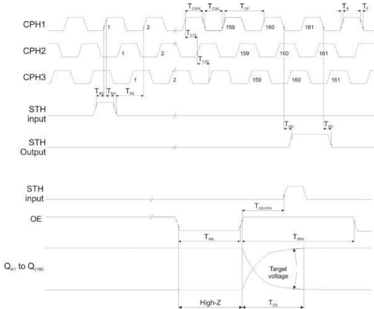
Fig. 7 Timing
