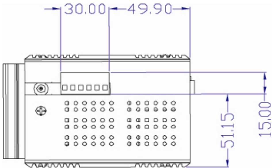
Figure 2.4: Top View of EKI-7626C/7626CI
