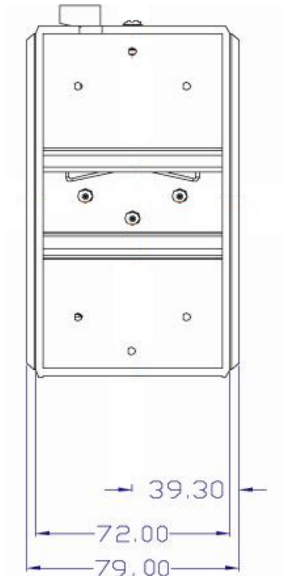
Figure 2.3: Rear View of EKI-7626C/7626CI
