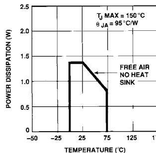
20-Pin SOL Maximum Power Dissipation vs Ambient Temperature
