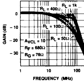
Gain vs Frequency
