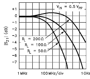
Frequency Response vs RLOAD
