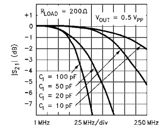
|S21| vs CLOAD with Recommended RS
