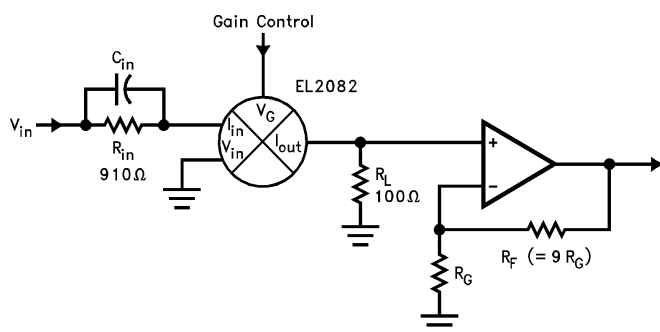
FIGURE 1. EL2082 + OP-AMP
