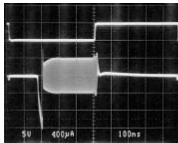
Enable Pin Response
