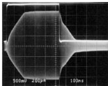
Gain Pin Transient Response
