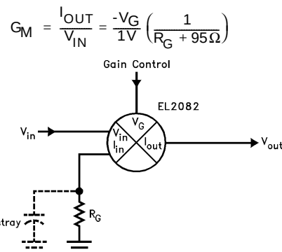
FIGURE 5. THE V_{IN} PIN USED AS SIGNAL INPUT
