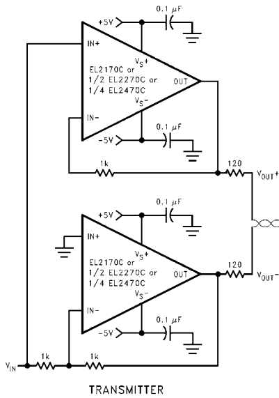
TRANSMITTER
