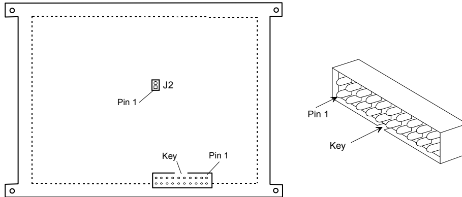
Figure 1. Data/Power Connector
