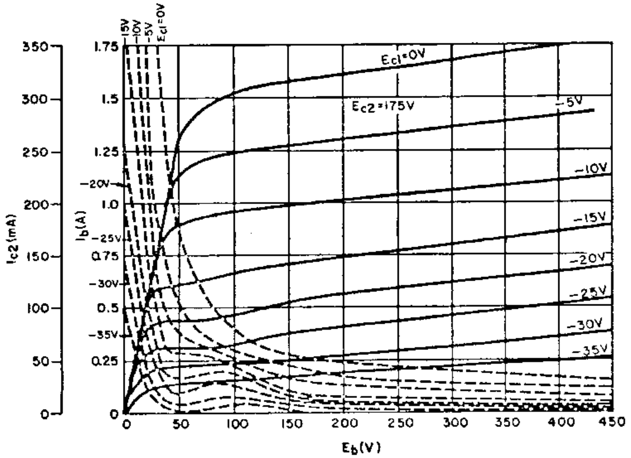
Plate Characteristics
