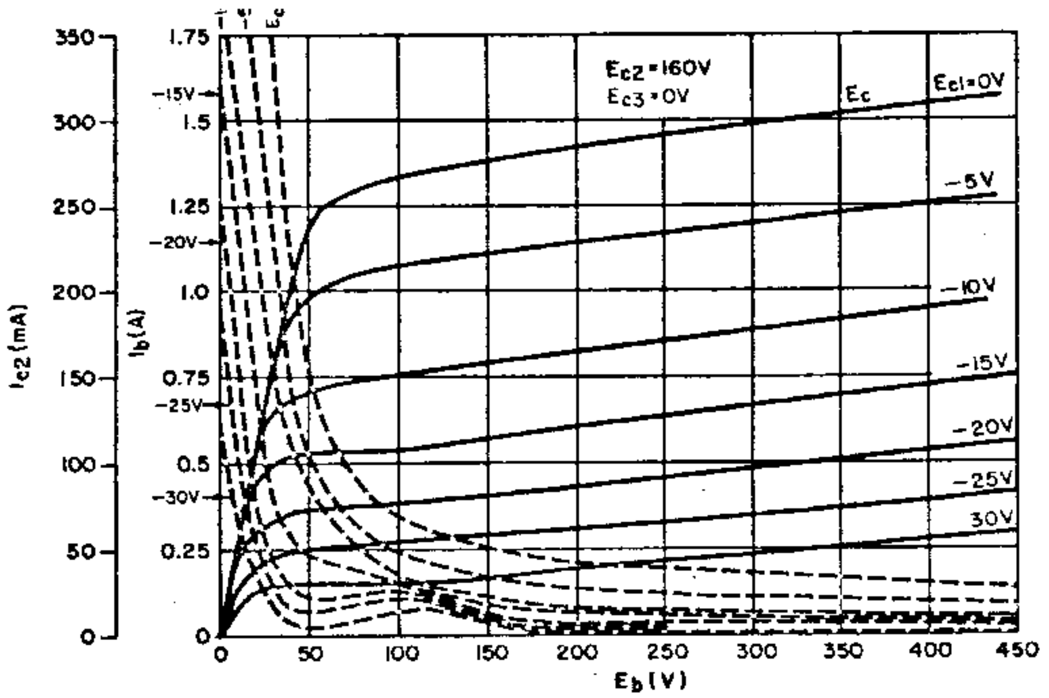
Plate Characteristics
