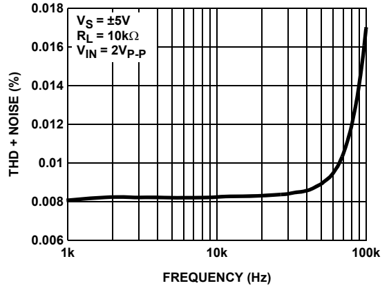
FIGURE 2. TOTAL HARMONIC DISTORTION + NOISE vs FREQUENCY
