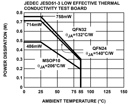
FIGURE 20. PACKAGE POWER DISSIPATION vs AMBIENT TEMPERATURE
