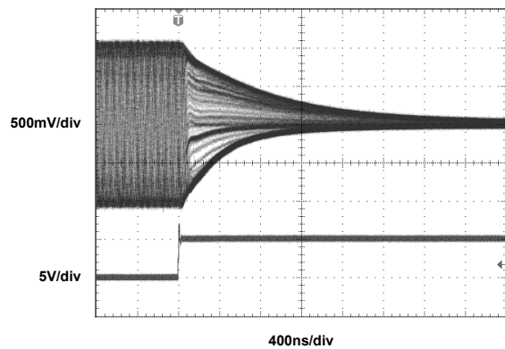
Disable Response
