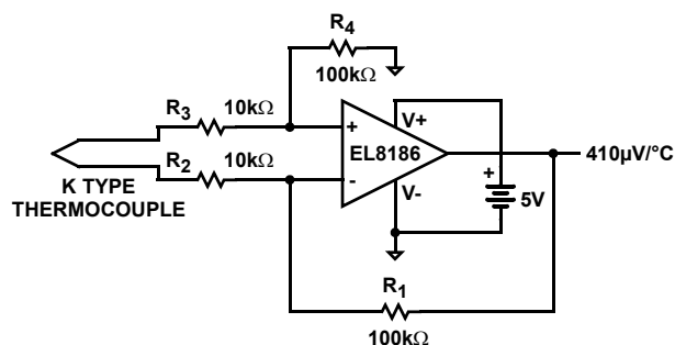
FIGURE 21. THERMOCOUPLE AMPLIFIER
