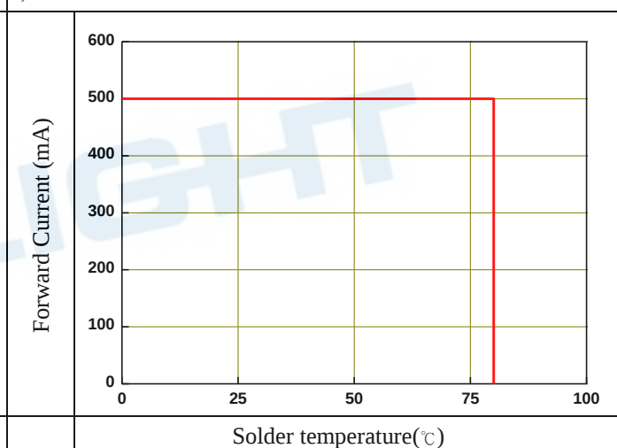
Forward Current Derating Curve, Derating based on
