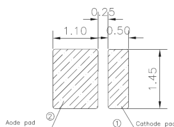
Soldering patterns
