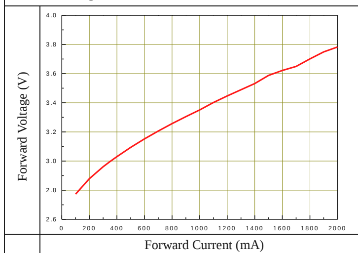
Forward Voltage vs. Forward Current ( T_{\text{solder pad}}=25^{\circ}\text{C} )
