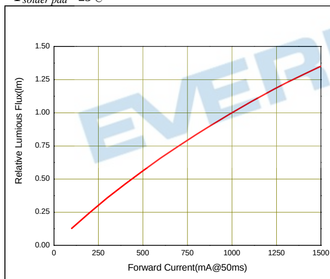
Luminous Flux vs Forward Current,
