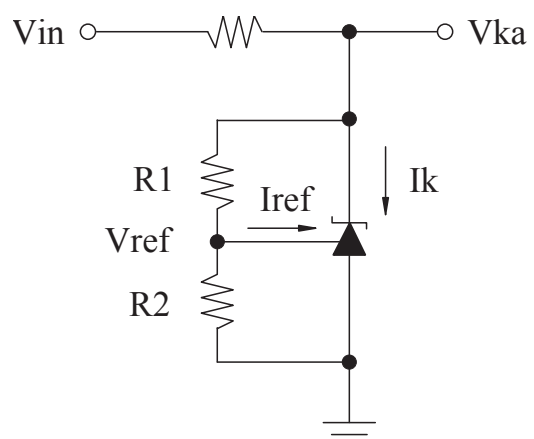
Test circuit 2 : V_{ka}>V_{ref}
