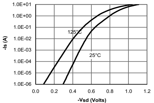
Figure 6: Body-Diode Characteristics
