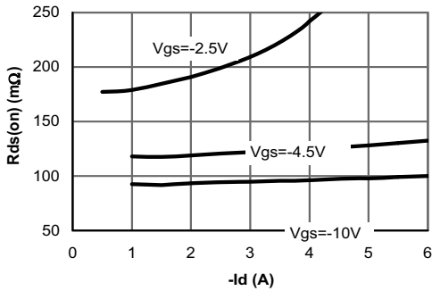
Figure 3: On-Resistance vs. Drain Current and Gate Voltage
