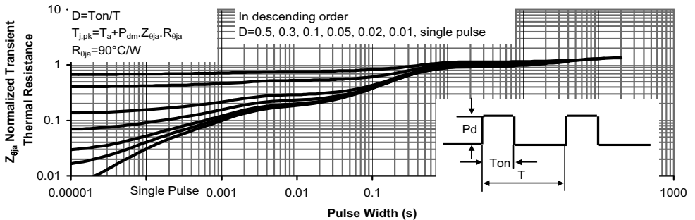
Figure 11: Normalized Maximum Transient Thermal Impedance
