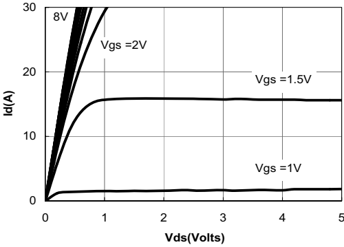
Figure 1: On-Regions Characteristics
