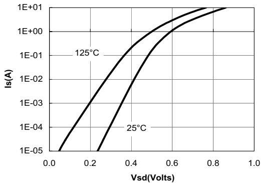
Figure 6: Body-Diode Characteristics
