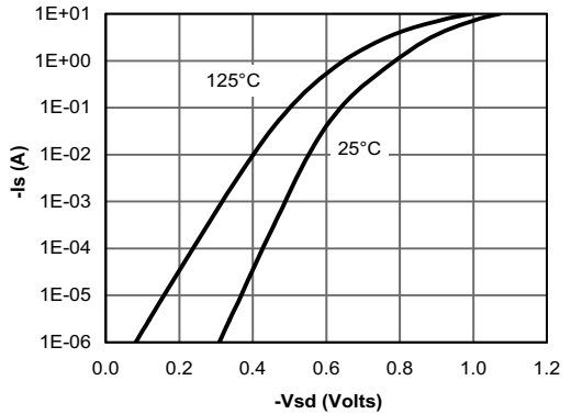
Figure 6: Body-Diode Characteristics
