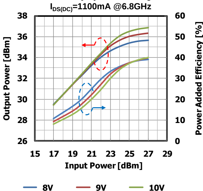
Input Power vs. Output Power, Power Added Efficiency by Drain Voltage I_{DS(DC)}=1100\text{mA} @6.8GHz
