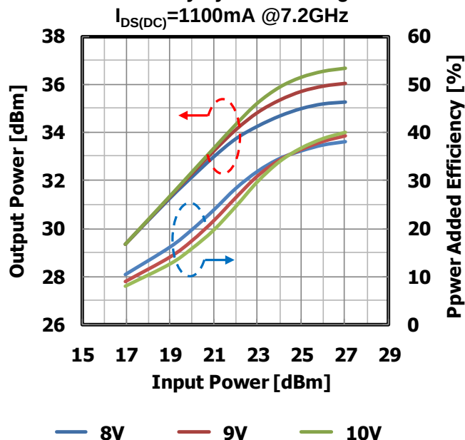
Input Power vs. Output Power, Power Added Efficiency by Drain Voltage I_{DS(DC)}=1100\text{mA} @7.2GHz
