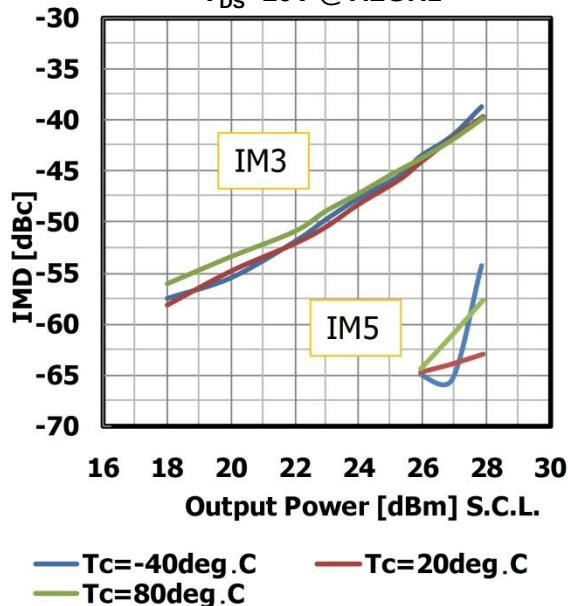
IMD Performance vs. Output Power by Temperature V_{DS}=10V @7.2GHz
