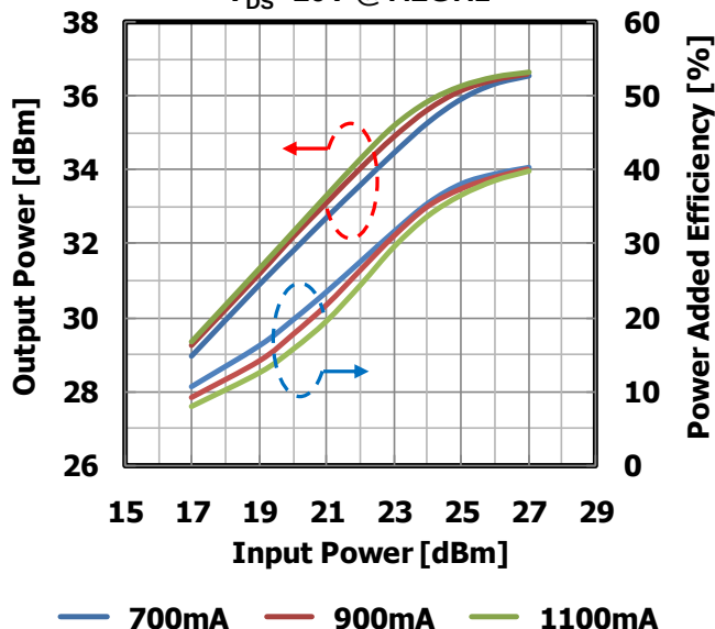
Input Power vs. Output Power, Power Added Efficiency by Quiescent Drain Current V_{DS}=10V @7.2GHz
