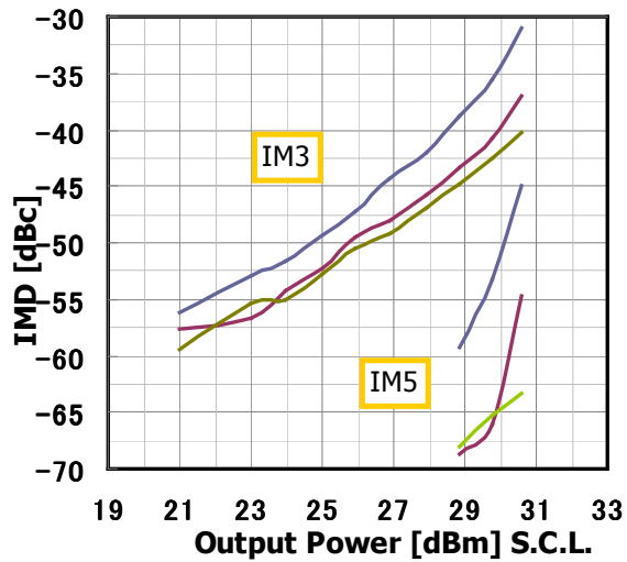
IMD Performance vs. Output Power by Drain Voltage I_{DS(DC)} = 2200\text{mA} @ 7.9\text{GHz}
