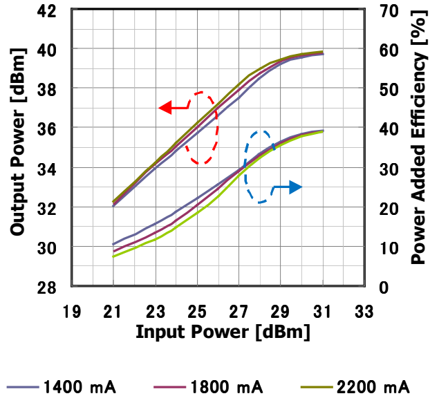
Input Power vs. Output Power, Power Added Efficiency by Quiescent Drain Current V_{DS}=10V @7.5GHz
