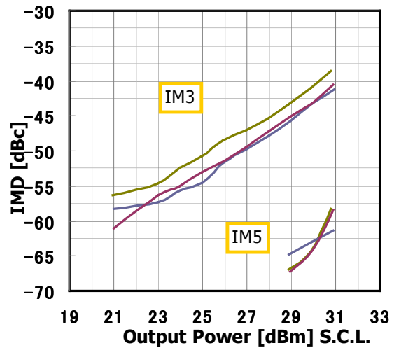
IMD Performance vs. Output Power by Temperature
