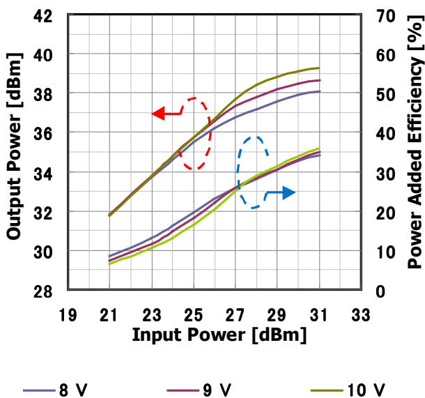
Input Power vs. Output Power, Power Added Efficiency by Drain Voltage I_{DS(DC)} = 2200\text{mA} @7.9GHz
