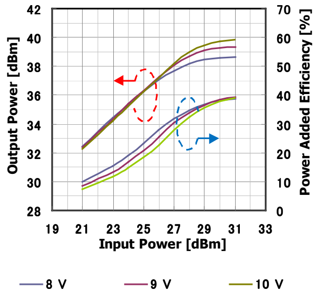
Input Power vs. Output Power, Power Added Efficiency by Drain Voltage I_{DS(DC)} = 2200\text{mA} @7.5GHz
