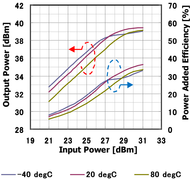
Input Power vs. Output Power, Power Added Efficiency by Temperature V_{DS}=10V I_{DS(DC)}=2200mA @7.9GHz
