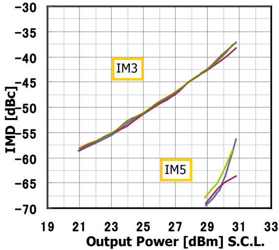
IMD Performance vs. Output Power by Drain Voltage I_{DS(DC)} = 2200\text{mA} @ 7.1\text{GHz}
