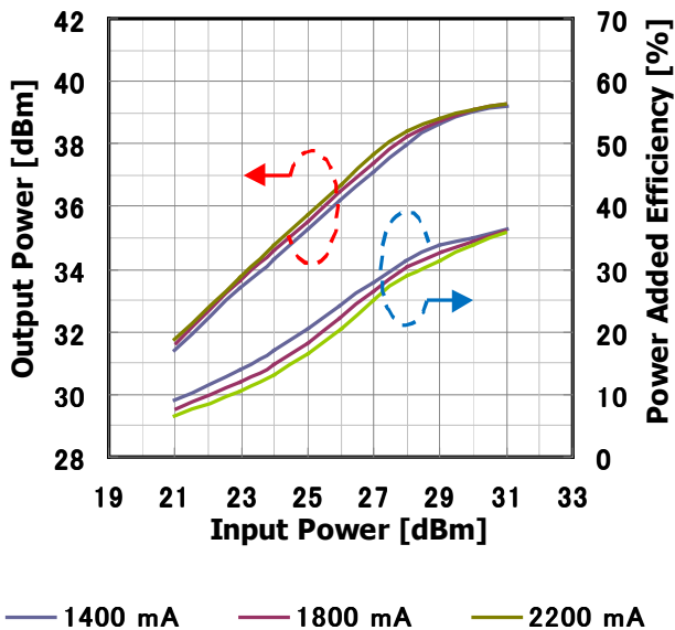
Input Power vs. Output Power, Power Added Efficiency by Quiescent Drain Current V_{DS}=10V @7.9GHz
