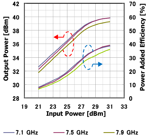
Input Power vs. Output Power, Power Added Efficiency V_{DS}=10V, I_{DS(DC)}=2200mA
