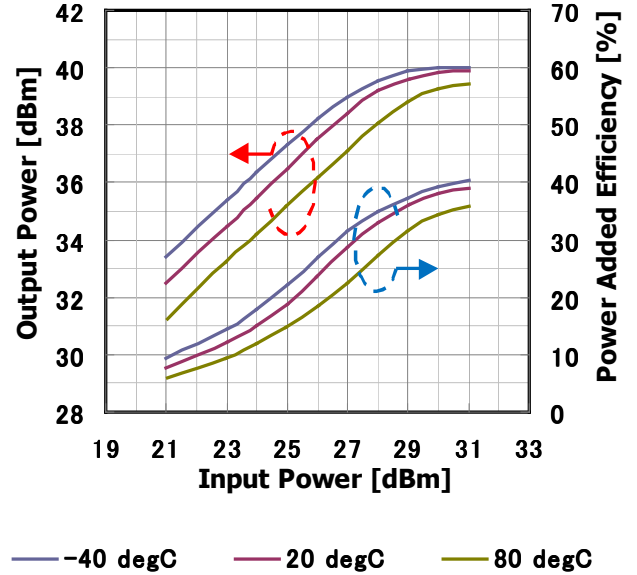
Input Power vs. Output Power, Power Added Efficiency by Temperature V_{DS}=10V I_{DS(DC)}=2200mA @7.5GHz
