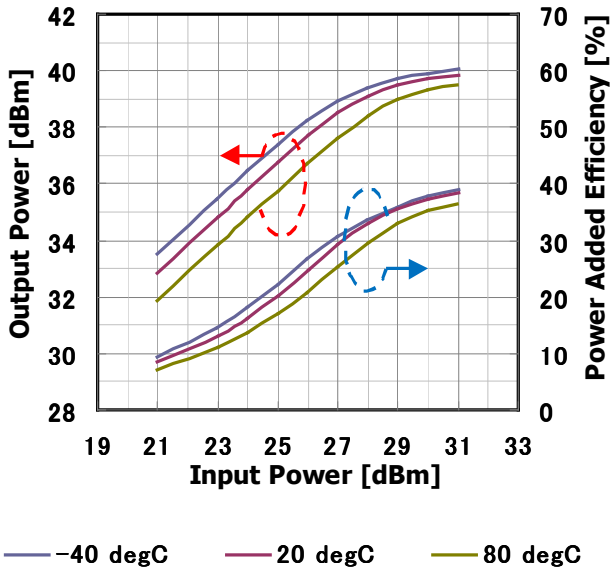
Input Power vs. Output Power, Power Added Efficiency by Temperature V_{DS}=10V I_{DS(DC)}=2200mA @7.1GHz
