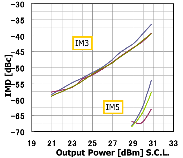
IMD Performance vs. Output Power by Drain Voltage I_{DS(DC)} = 2200\text{mA} @ 7.5\text{GHz}
