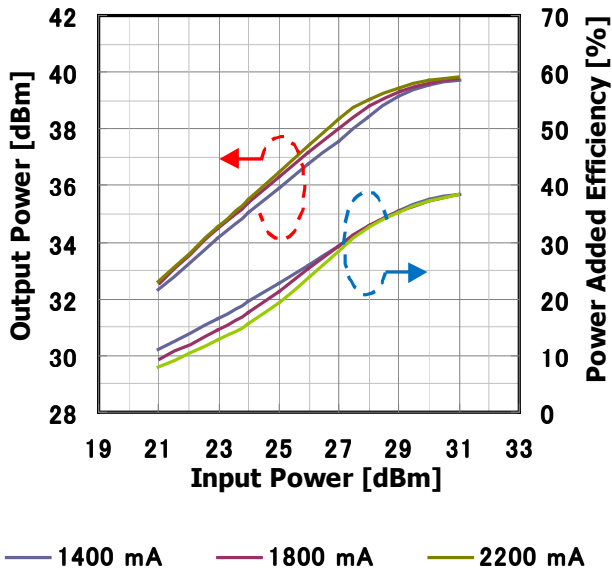
Input Power vs. Output Power, Power Added Efficiency by Quiescent Drain Current V_{DS}=10V @7.1GHz
