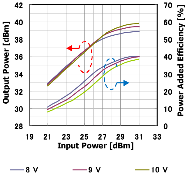
Input Power vs. Output Power, Power Added Efficiency by Drain Voltage I_{DS(DC)} = 2200\text{mA} @7.1GHz
