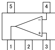
SOT-25 (TOP VIEW)
