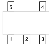
SC-70-5 (TOP VIEW)
