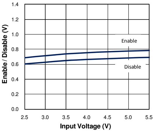
Enable/Disable v.s. Input Voltage
