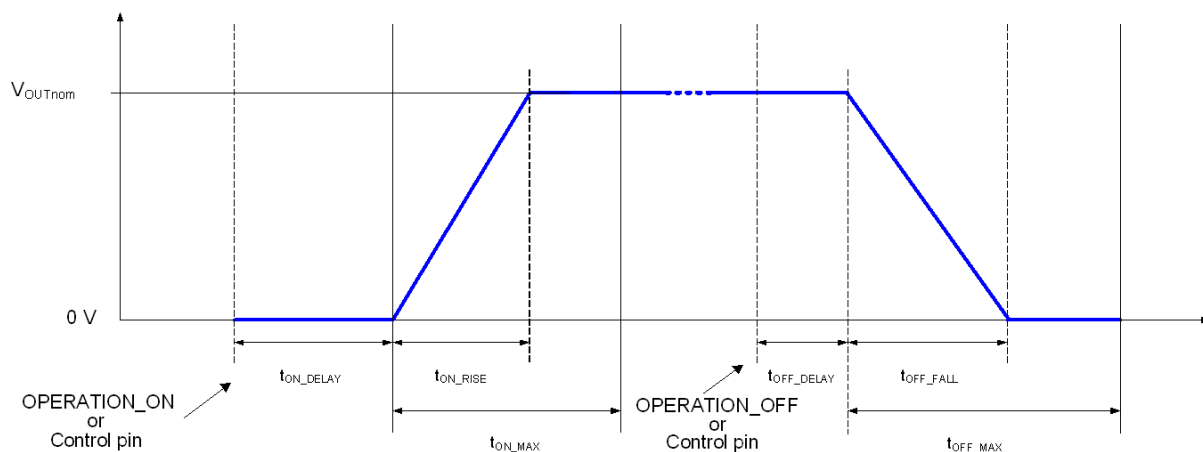
Figure 6: Power Sequencing
