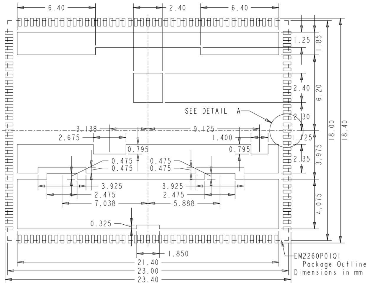
Figure 19: Recommended PCB Footprint (Top View)
