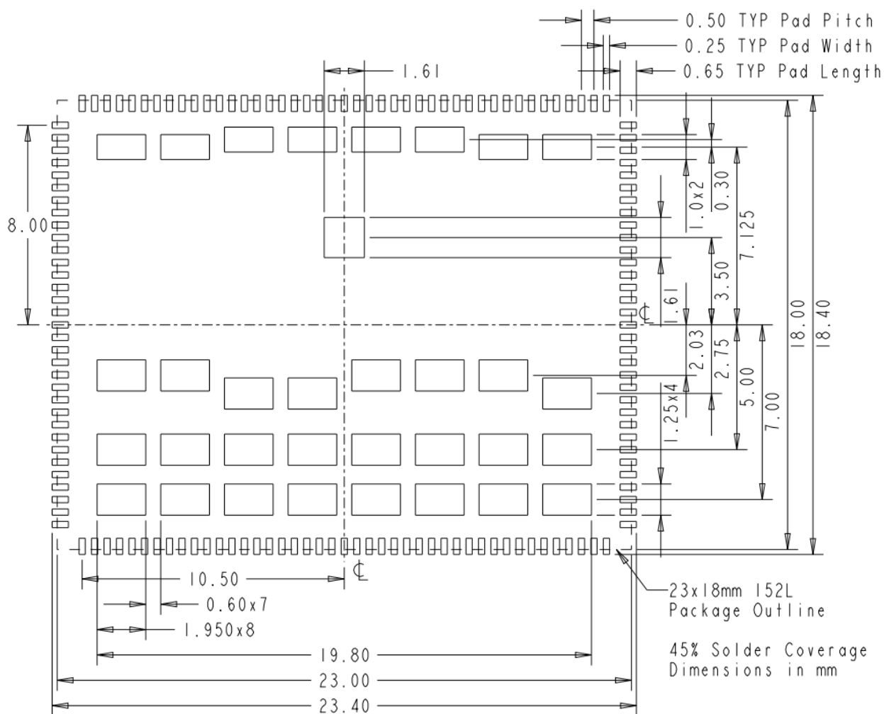
Figure 22: 45% Solder Stencil Aperture Dimensions
