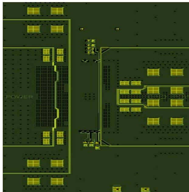
Figure 17: Backside Decoupling
