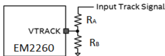
Figure 11: VTRACK Sense Circuitry with Resistor Divider
