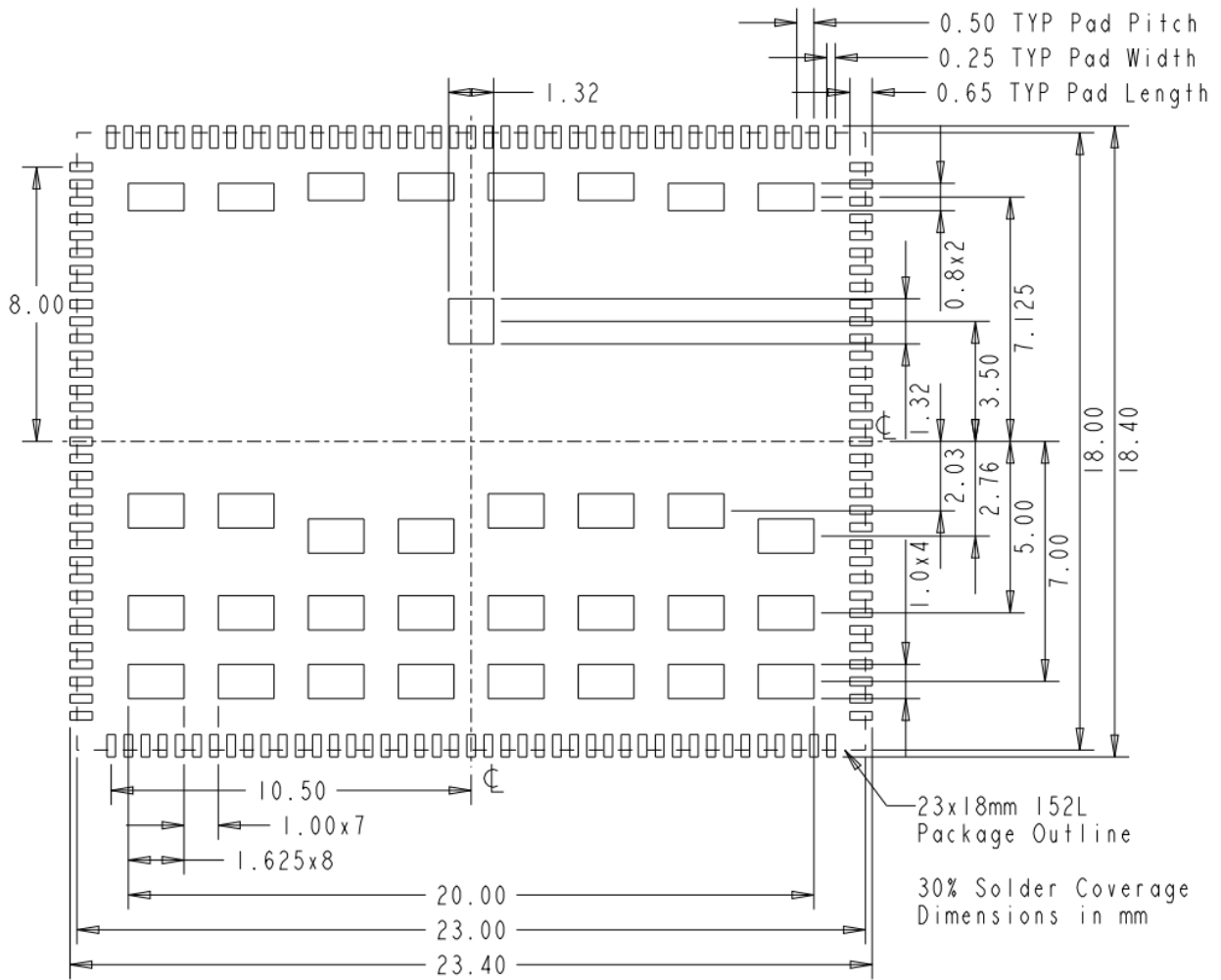
Figure 21: 30% Solder Stencil Aperture Dimensions
