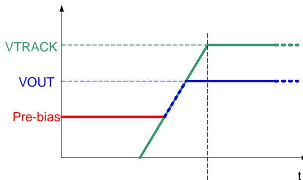
Figure 7: Power Sequencing Using VTRACK With Bias Voltage On VOUT
