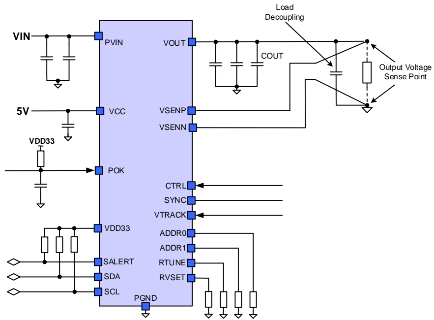
Figure 14: Recommended Application Circuit
