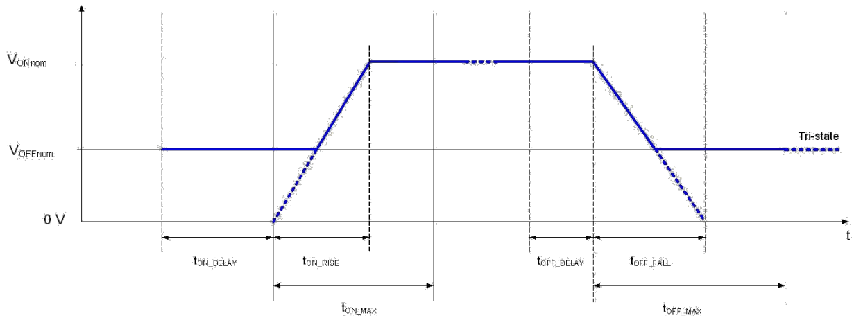
Figure 6: Power Sequencing with Non-Zero Off Voltage
