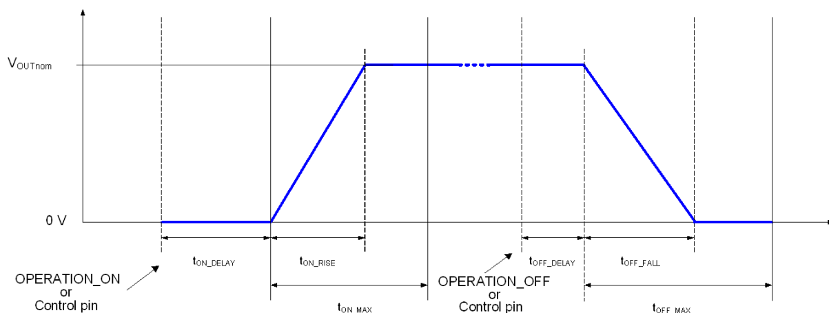
Figure 5: Power Sequencing
